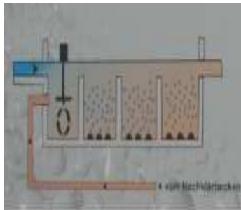
[Graphik 8: Biolog. Reinigung]
